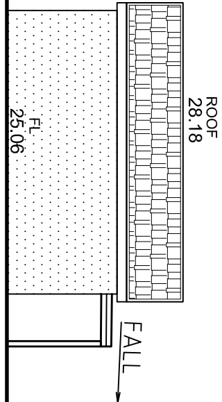
Northeastern Elevation
